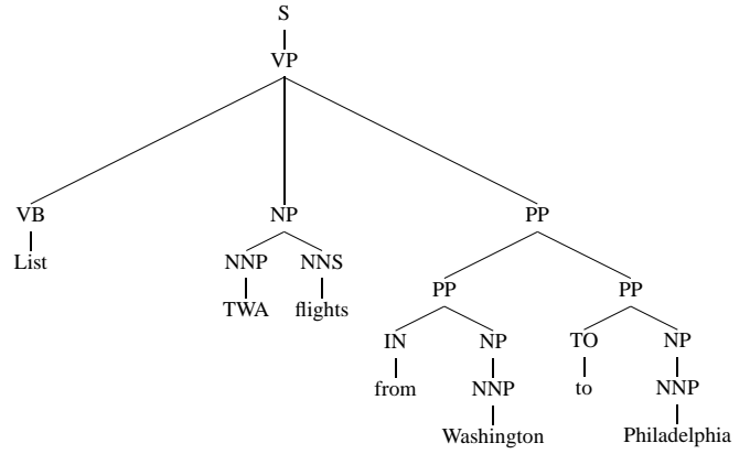
Fig. 3. Charniak Parse Tree
