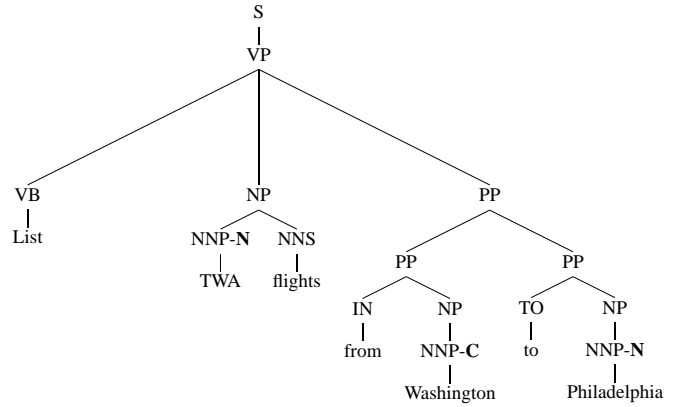
Fig. 4. Syntactic Semantic Tree
