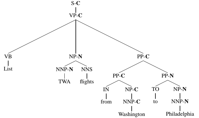
Fig. 5. Syntactic Semantic Tree with percolating concepts
