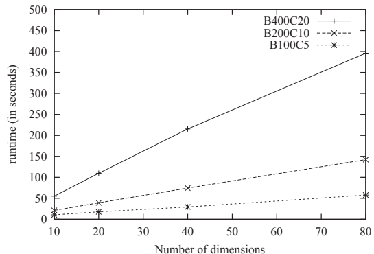
Figure 7: Scalability with Data Dimensionality (stream_speed=2000)
