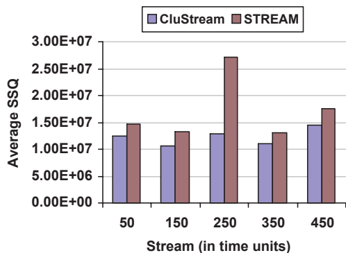
Figure 3: Quality comparison (Charitable Donation dataset, horizon=4, stream_speed=200)
