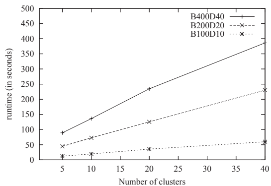
Figure 8: Scalability with Number of Clusters (stream_speed=2000)
