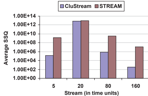
Figure 1: Quality comparison (Network Intrusion dataset, horizon=1, stream_speed=2000)
