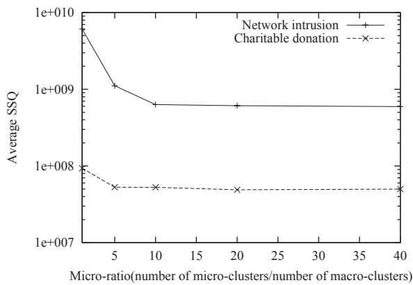
Figure 9: Accuracy Impact of Micro-clusters
