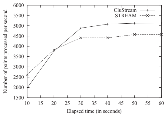
Figure 6: Stream Processing Rate (Network Intrusion dataset, stream_speed=2000)
