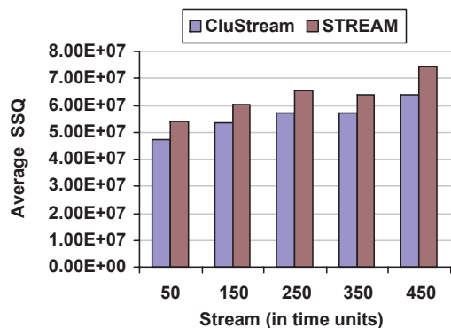
Figure 4: Quality comparison (Charitable Donation dataset, horizon=16, stream_speed=200)
