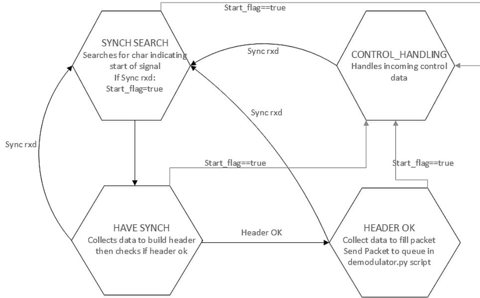
Figure 4: frame synchronization state machine implemented in “frame_sink” block.
