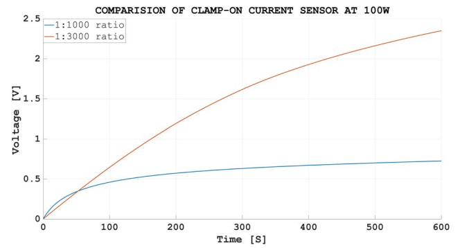
Fig. 4. Super capacitor voltage trend using different transformer ratio. Contrary to the expected behavior, the CT sensor with a higher number of turns better match the energy harvesting system, leading to a higher efficiency in charging the super-capacitor.
