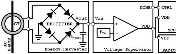
Fig. 3. Power supply control system block schematics.
