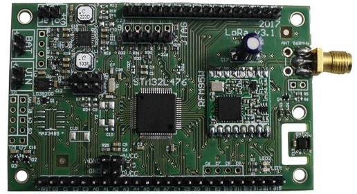
Fig. 2. Assembled board with microcontroller and radio.
