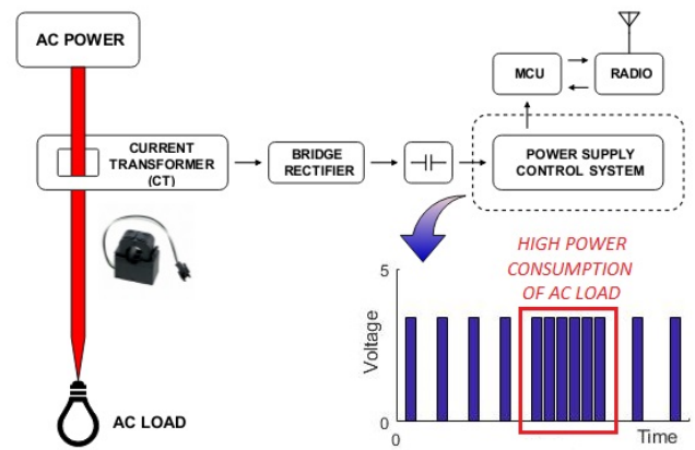
Fig. 1. Block diagram of the node architecture.
