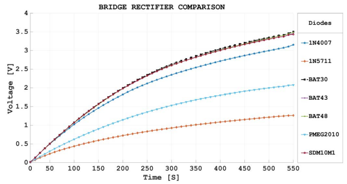
Fig. 6. Super-capacitor charge profile for a 130 W load using different rectifier bridges. The dashed line (BAT30), represent the chosen solution. We chose this diode as more efficient at lower load, in order to extend the functionalities of the meter also at lower primary loads.
