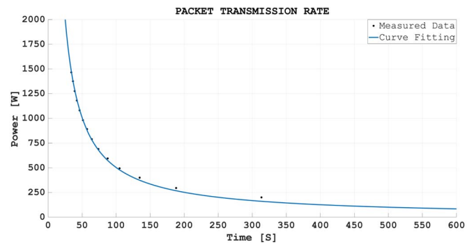
Fig. 7. Packet transmission rate at different primary loads.
