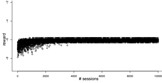
(a) 0% exploration, 100% exploitation: learner does not find optimal dialogue strategy
