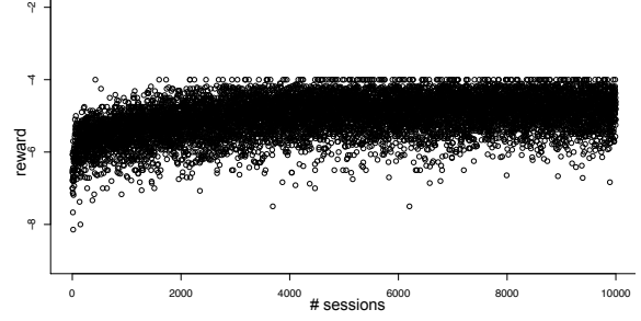
(b) 20% exploration, 80% exploitation: noticeable increase in reward, hitting upper bound
