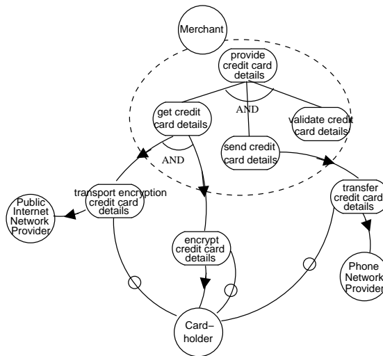
Fig. 8. Internet Shopping à la TLS/HTTPS
