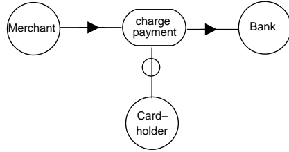
Fig. 5. Extended dependency diagram
