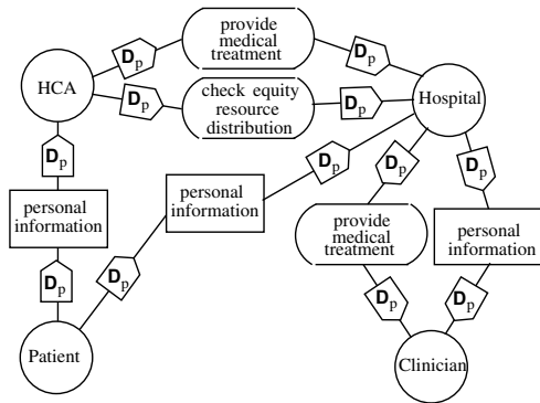
Fig. 5 Early Requirements TM implementation
