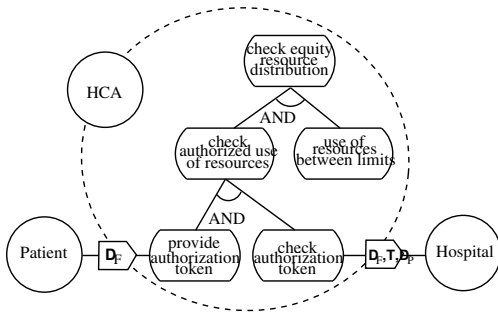
Fig. 7 Goal Diagram for the HCA
