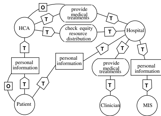
Fig. 8 Late Requirements trust model
