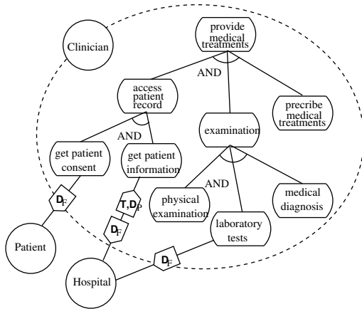
Fig. 6 Goal Diagram for the Clinician
