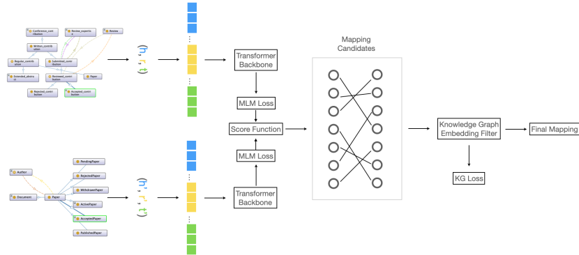
Fig. 1. The overall framework of AMD. Here, inputs are sub-graphs of source and target ontologies. It learns language and knowledge embeddings by using a novel relation attention mechanism. Ontology matching tasks are solved using the outputs of masked language model, and final mappings are selected from candidate sets by knowledge graph embedding..
