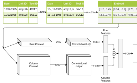
Fig. 1: TableCNN Architecture.
