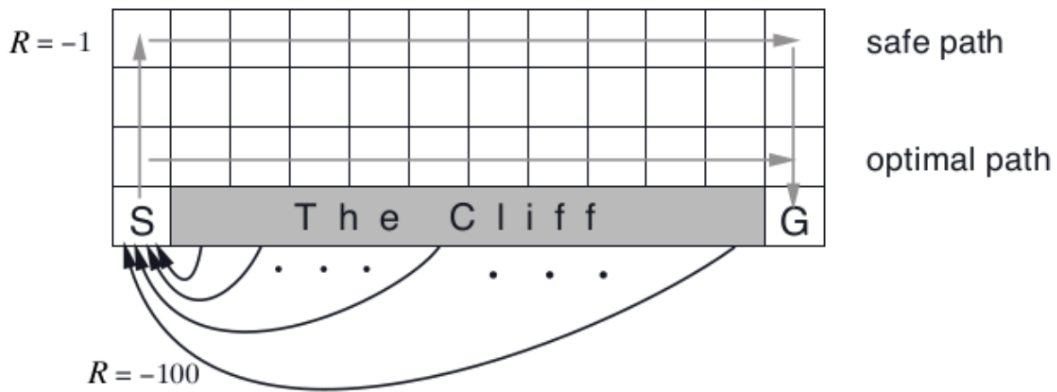
cliff walking example
