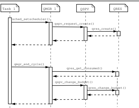
Figure 5. Interaction between the QMGR, the QSPV and the QRES modules.
