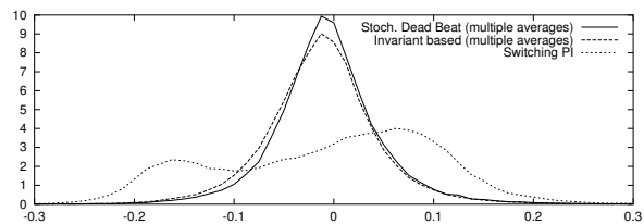
Figure 7. Scheduling error PDF achieved by switching PI, invariant-based and SDB controllers.
