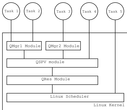
Figure 4. OCERA soft RT architecture.
