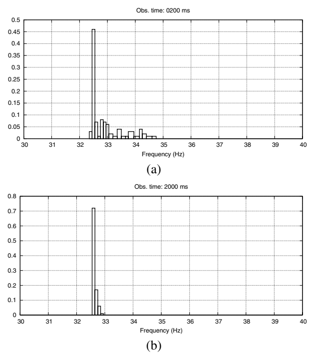
Figure 11. PMF of the frequency detected by LFS++ for mplayer at varying tracing times.
