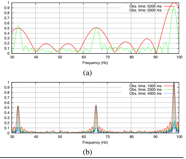
Figure 10. Normalized frequency-transform of the events obtained by tracing mplayer at varying tracing time.
