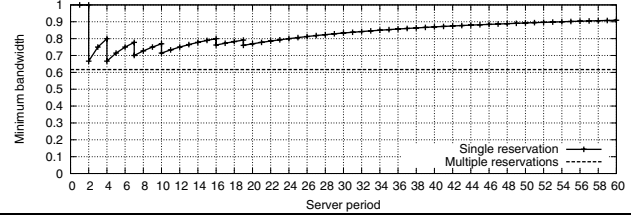
Figure 2. Minimum bandwidth required to schedule in a single reservation three tasks. The task parameters are C_1 = 3 ms, P_1 = 15 ms, C_2 = 5 ms, P_2 = 20 ms, C_3 = 5 ms, P_3 = 30 ms and the cumulative utilisation is \approx 62\% .
