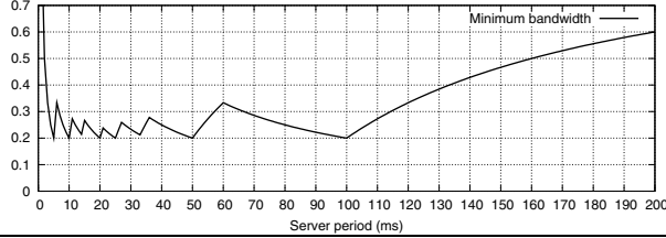
Figure 1. Fraction of CPU Q_i^s/T_i^s required to correctly schedule a real-time task with 20% utilisation C = 20 ms, P = 100 ms.
