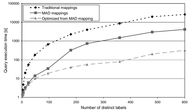
Figure 8: Impact of MAD mappings for Metadata-to-Data exchange.
