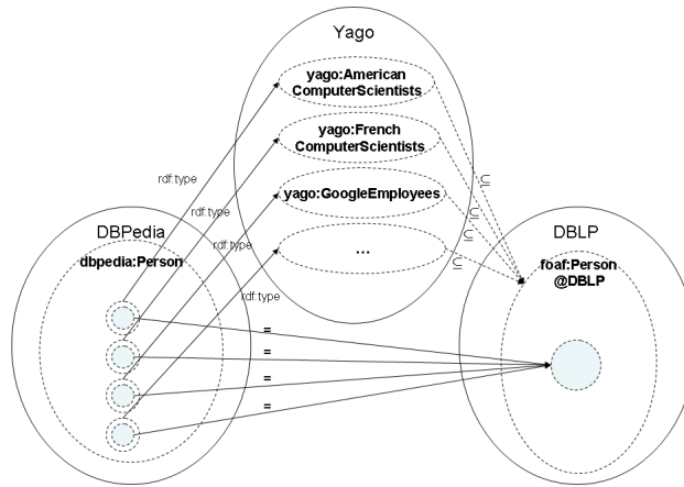
Fig. 1. DBPedia and DBLP: exploiting schema-level links with third-party datasets. Solid arrows show existing owl:sameAs (=) and rdfs:type links. Dashed arrows represent discovered schema relations. The system identifies the subset of dbpedia:Person instances, which overlaps with DBLP foaf:Person instances, as a union of classes defined in YAGO.
