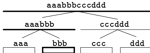
Figure 20: The hierarchical verification method for a pattern split in 4 parts. The boxes (leaves) are the elements which are really searched, and the root represents the whole pattern. At least one pattern at each level must match in any occurrence of the complete pattern. If the bold box is found, all the bold lines may be verified.
