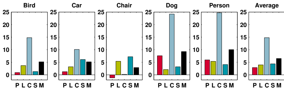
Figure 3. Relative improvement of undoing dataset bias LSM vs. undoing bias SVM [15].
