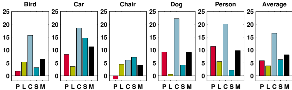
Figure 2. Relative improvement of undoing dataset bias LSM vs. the baseline LSM trained on all datasets at once (aggregated LSM). On all datasets at once (P: PASCAL, L: LabelMe, C: Caltech101, SUN: M: mean).
