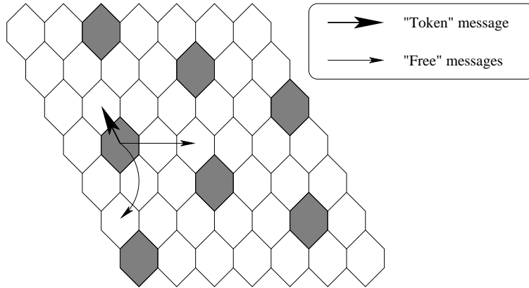
Figure 5: A multiple token-passing scheme
