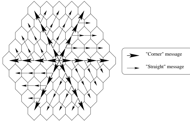
Figure 3: A local broadcasting scheme
