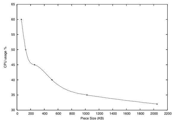
Fig. 3. CPU usage for varying piece sizes
