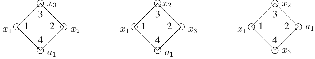
Figure 8: 3 possible placements of \underline{z} \stackrel{\text{def}}{=} \{x_1, x_2, x_3\} \cup \{a_1\} into a 4-qubit tile fraction with 2 horizontal and 2 vertical qubits. All 4! = 24 combinations are equivalent to one of them.
