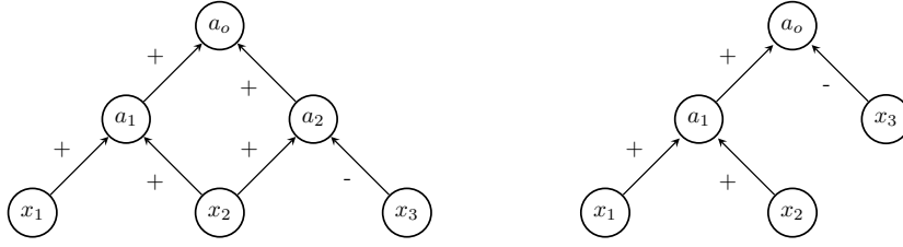
Figure 10: Two And-Inverter Graphs representing the function F(\underline{x}) = x_1 \wedge x_2 \wedge \neg x_3 .
