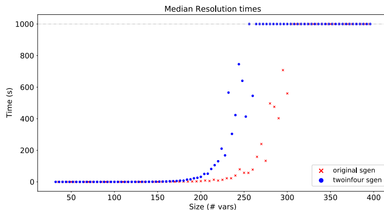
Figure 11: Median times for the best-performing SLS algorithm on two different variants of the SGEN problem on UBCSAT (SAPS). Timeout is marked with a gray line. The figure report times on a computer with a 8-core Intel® Xeon® E5-2407 CPU, at 2.20GHz.
