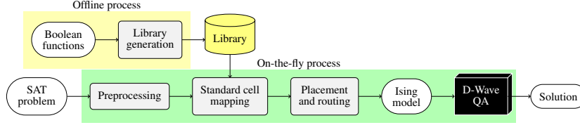
Figure 9: Graph of the encoding process.
