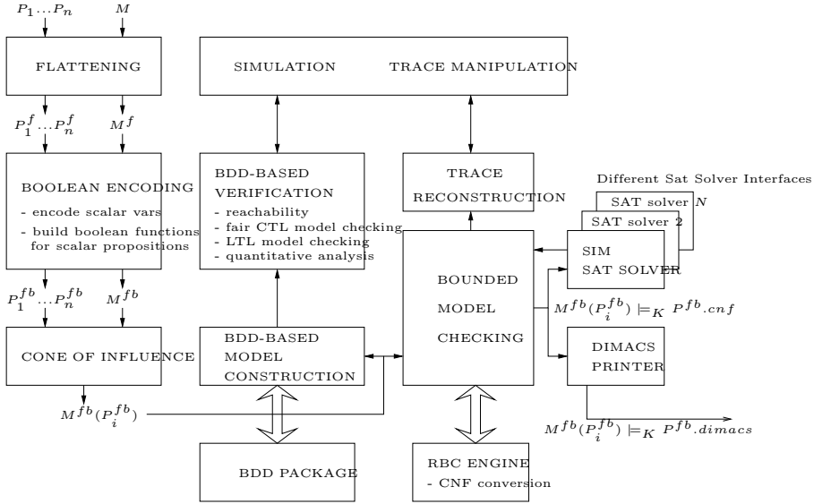
Fig. 1. The internal structure of NuSMV2
