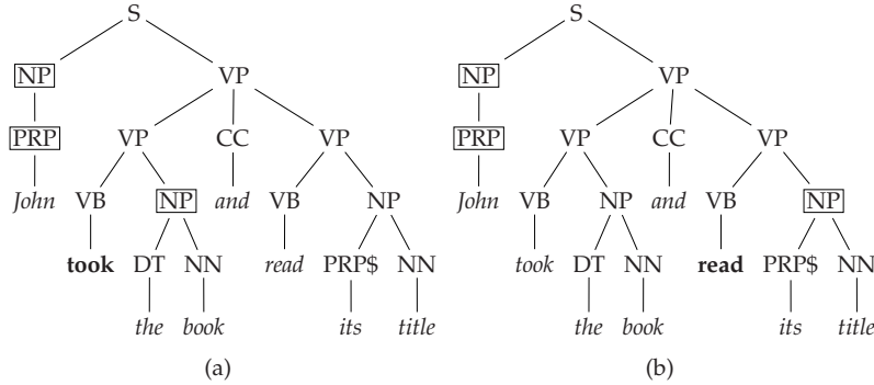
Figure 2 Positive (framed) and negative (unframed) examples of candidate argument nodes for the propositions (a) [Arg_0 \text{ John}] \text{ took } [Arg_1 \text{ the book}] \text{ and read its title} and (b) [Arg_0 \text{ John}] \text{ took the book and read } [Arg_1 \text{ its title}] .
