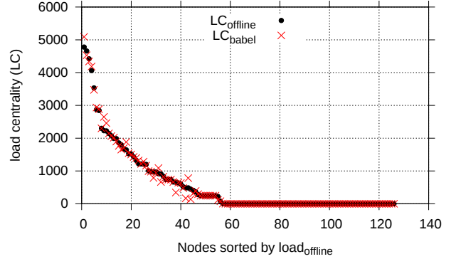
Figure 4. Comparison of LC computed on-line with babeld and off-line with networkx on the same topology computed by Babel
