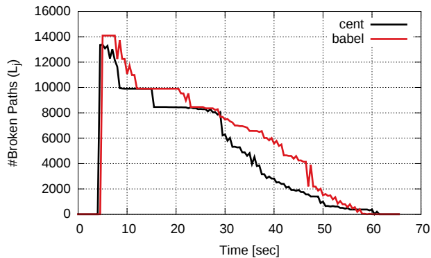
Figure 5. Comparison of the network loss in ninux topology after the failure of one of the most central nodes
