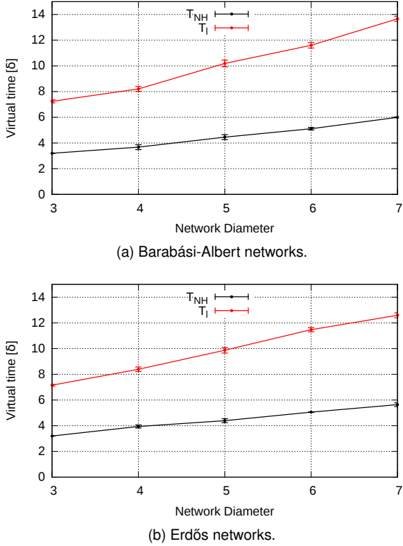
Figure 2. T_{NH} and T_l Vs network diameter, with 99% confidence interval, for Barabási-Albert and Erdős networks.
