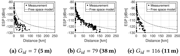
Figure 3: ESP vs. distance for selected gateways.
