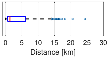
Figure 4: Variation of communication ranges for LoRa links.
