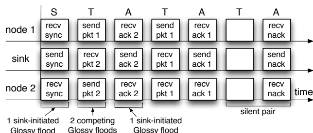
Figure 1. CRYSTAL in a nutshell.
